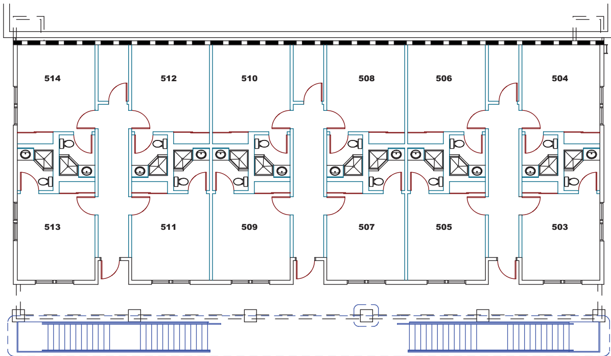
SECOND FLOOR
